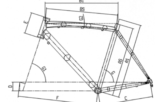
C2C - VIA NIRONE 7 Lady Alu
